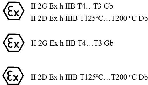
Figure 1.1.: EC ATEX mark inscribed on the manufacturer's plate.
